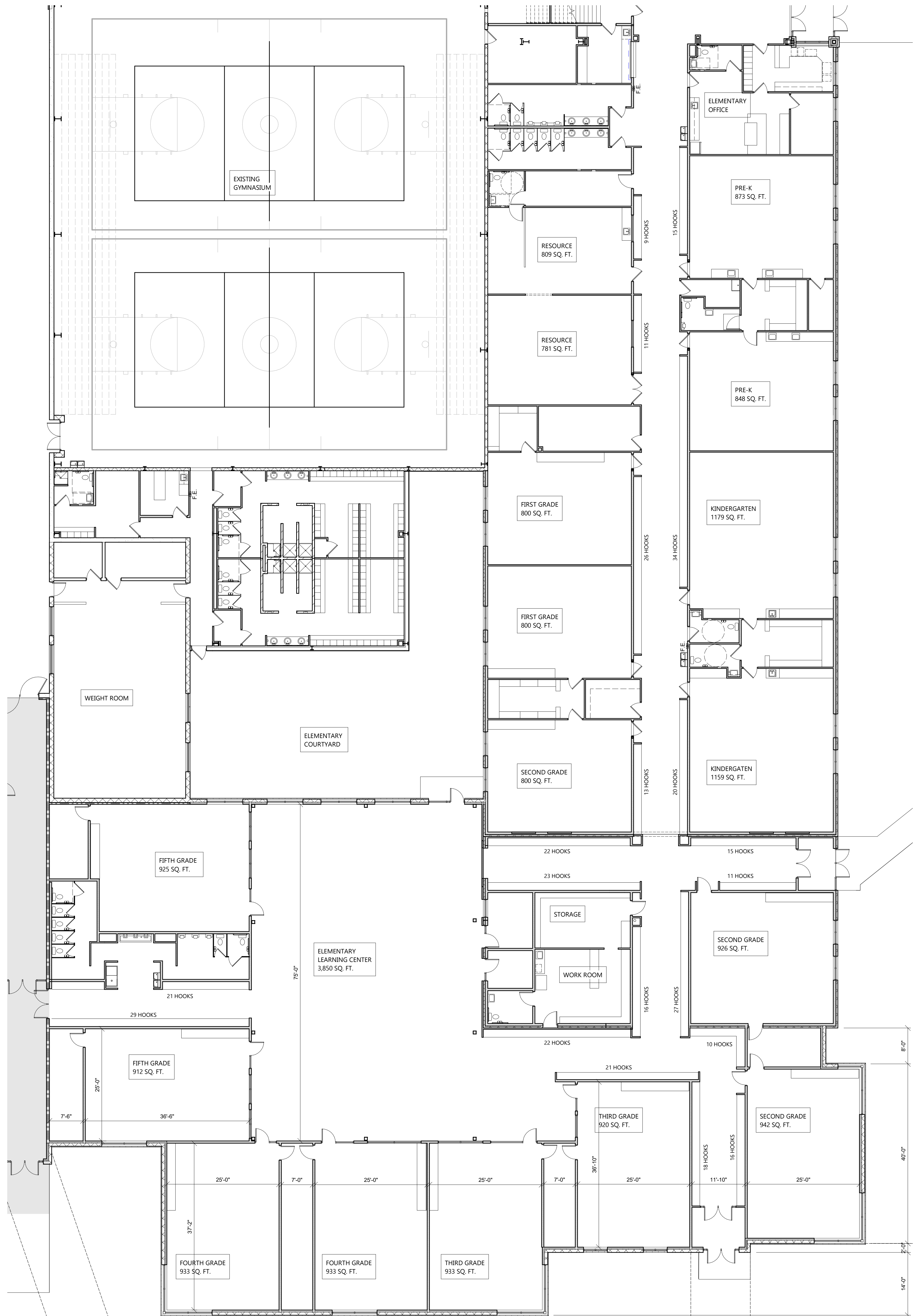
NORTH ELEMENTARY SCHOOL PLAN SCALE: 3/32" = 1'-0"
